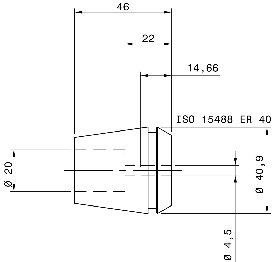
REGO-FIX 1140.04500
