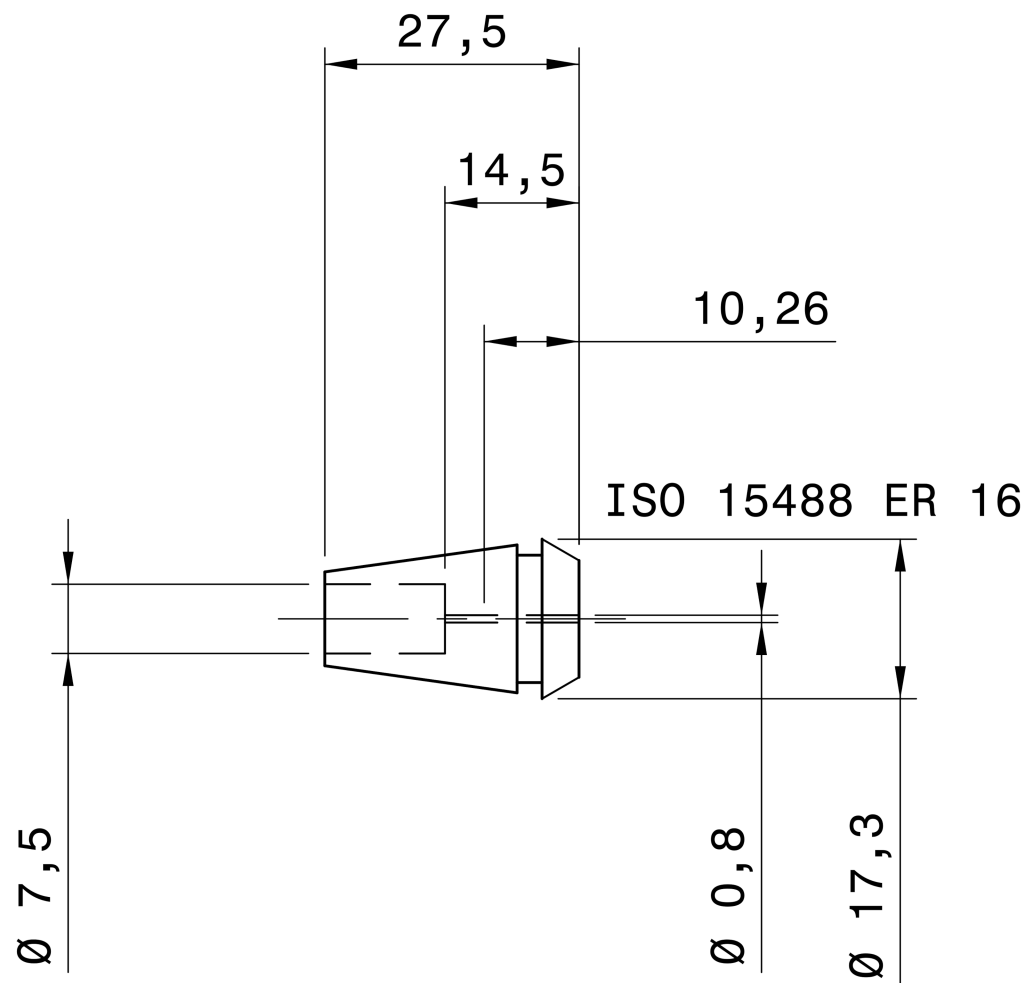
REGO-FIX 1316.00800
