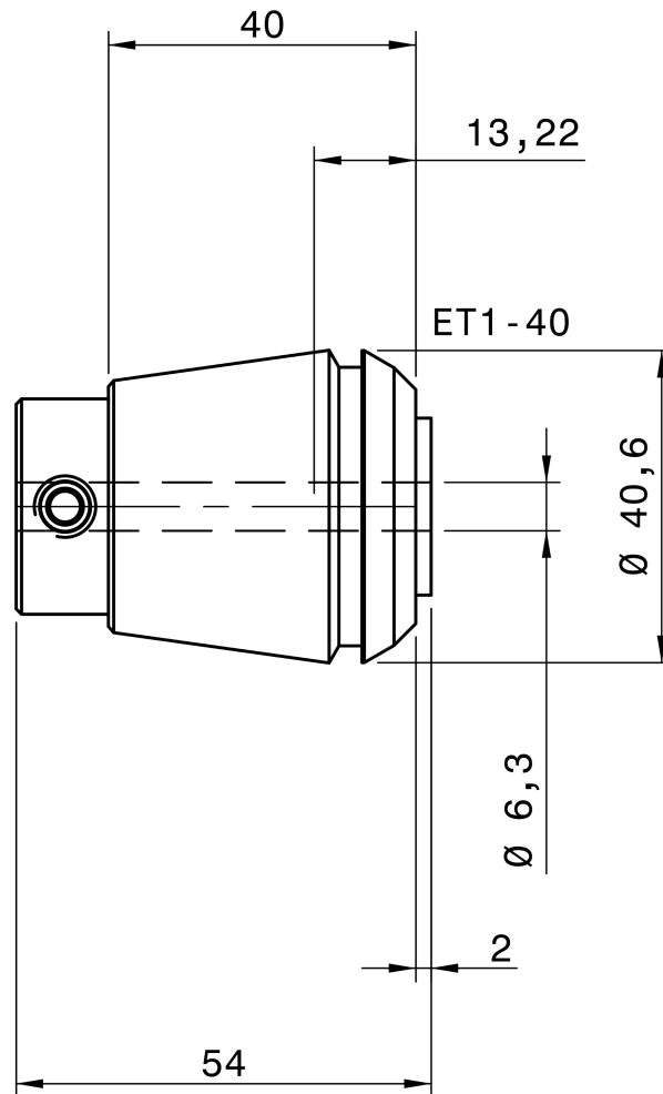
REGO-FIX 1540.06300
