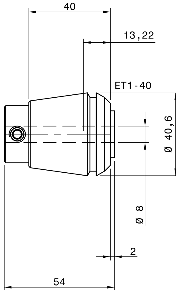
REGO-FIX 1540.08000
