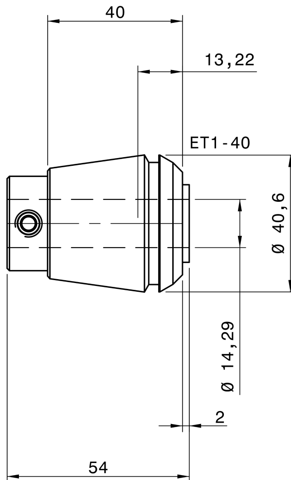
REGO-FIX 1540.14291
