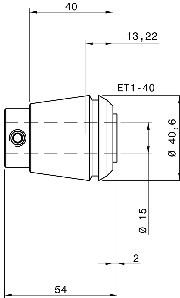
REGO-FIX 1540.15000
