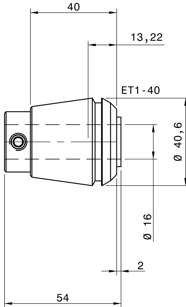
REGO-FIX 1540.16000
