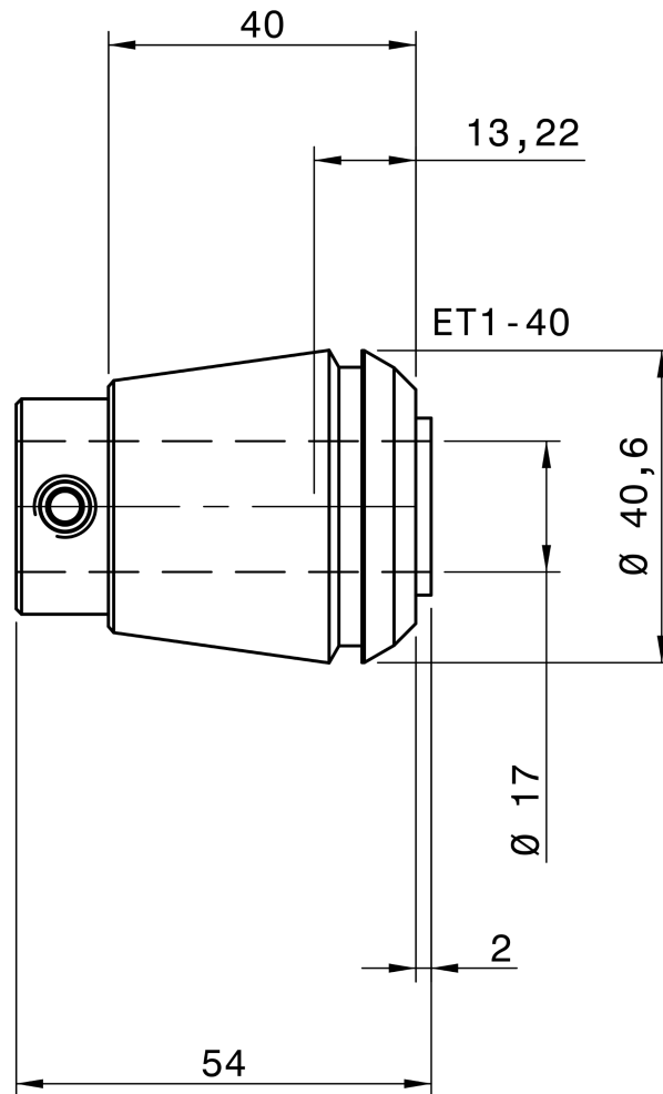
REGO-FIX 1540.17000
