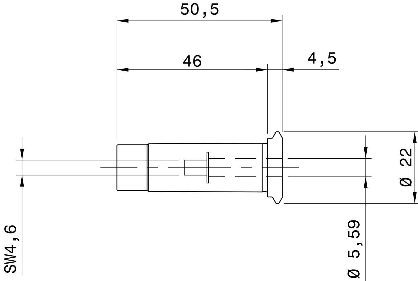
REGO-FIX 1715.05595
