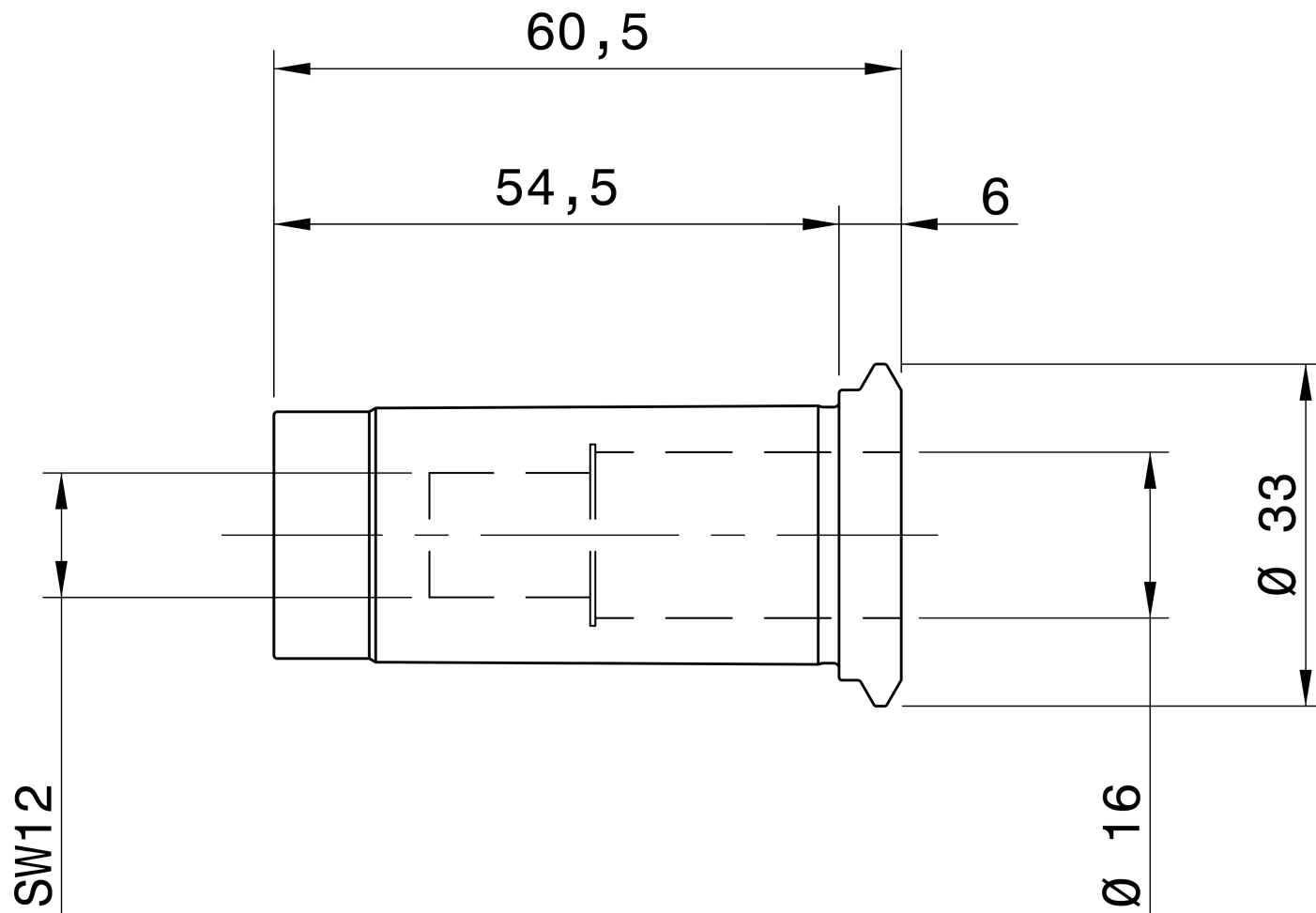
REGO-FIX 1725.16005
