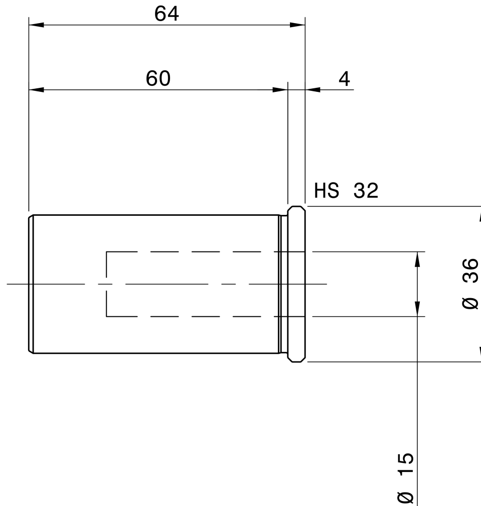
REGO-FIX 1932.15000
