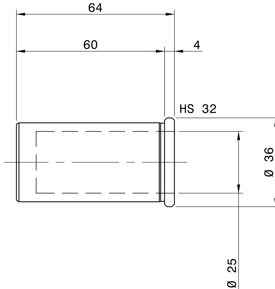
REGO-FIX 1932.25000
