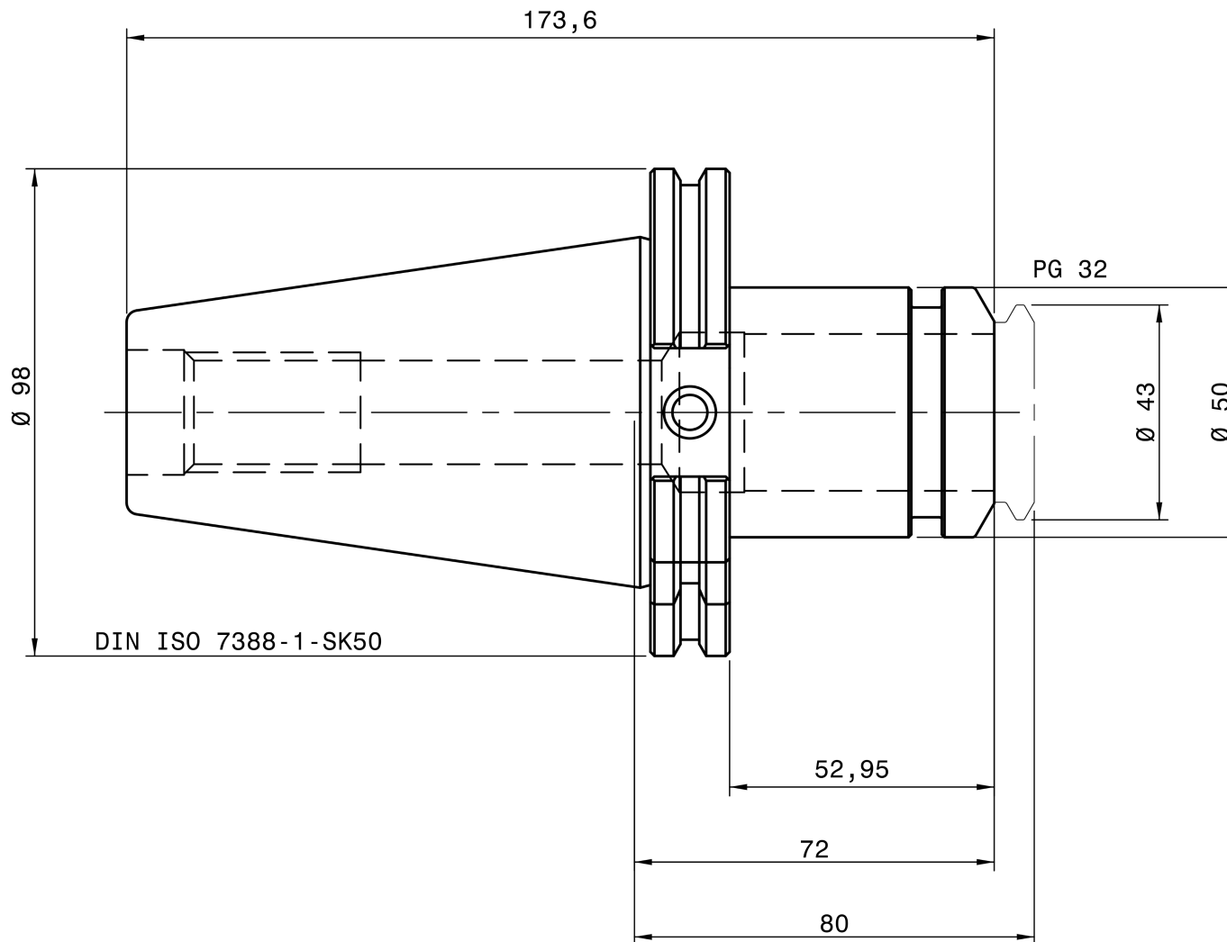
REGO-FIX 2250.73240
