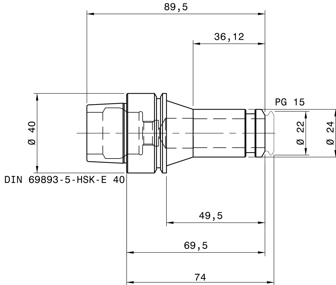
REGO-FIX 2540.71534
