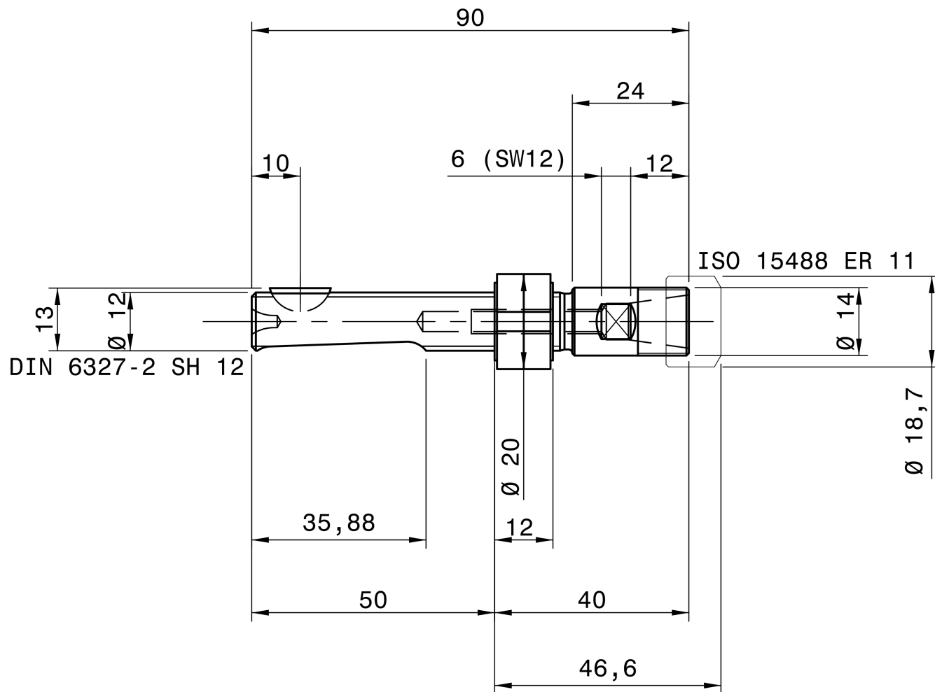
REGO-FIX 2612.11104
