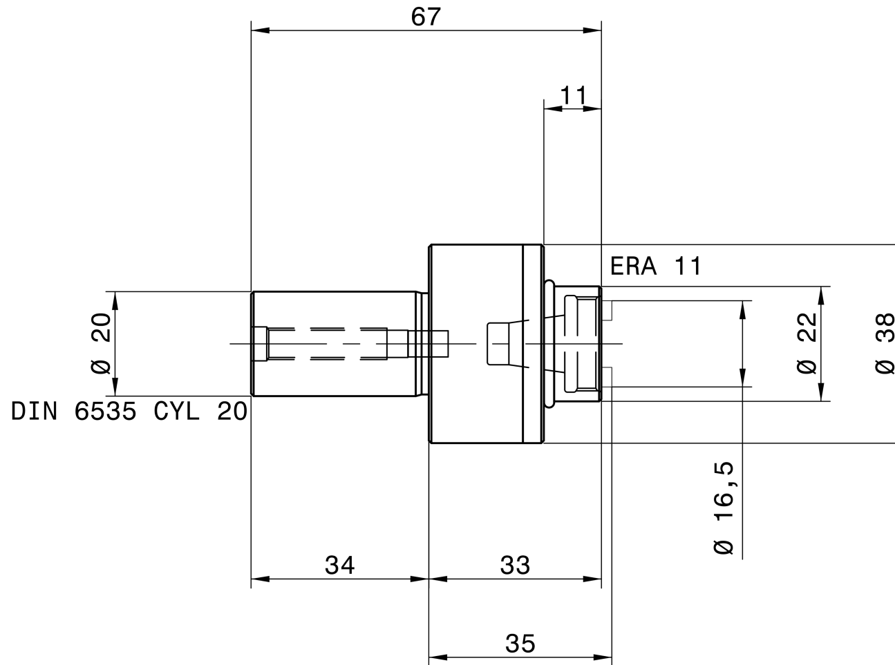
REGO-FIX 2620.91100
