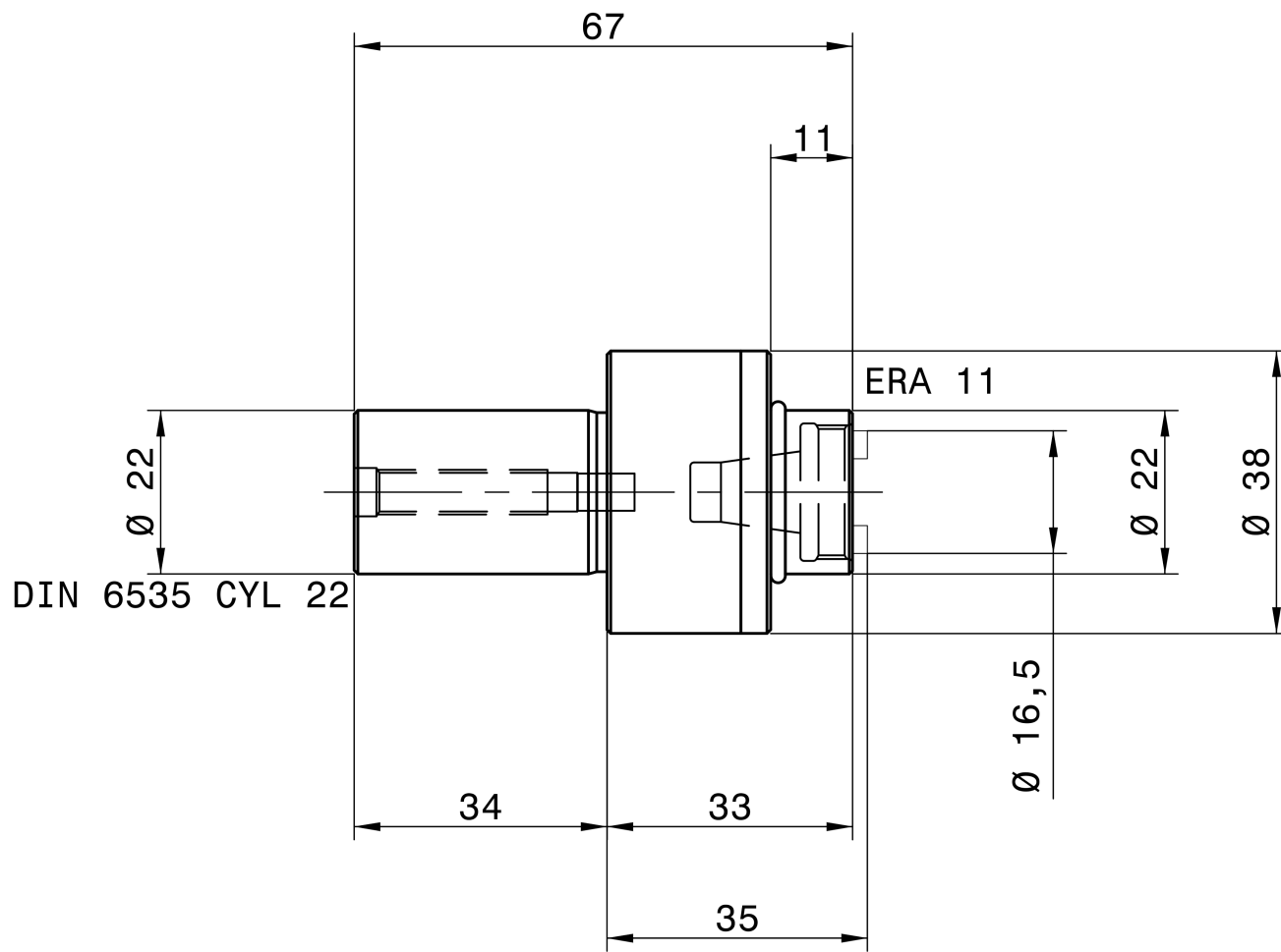
REGO-FIX 2622.91100
