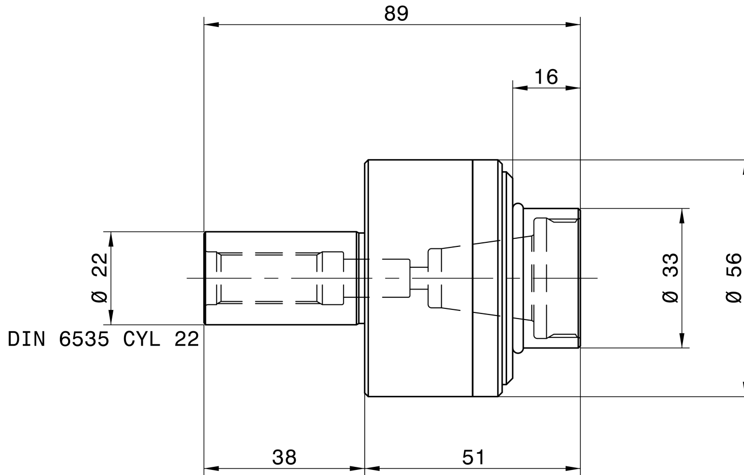
REGO-FIX 2622.92003
