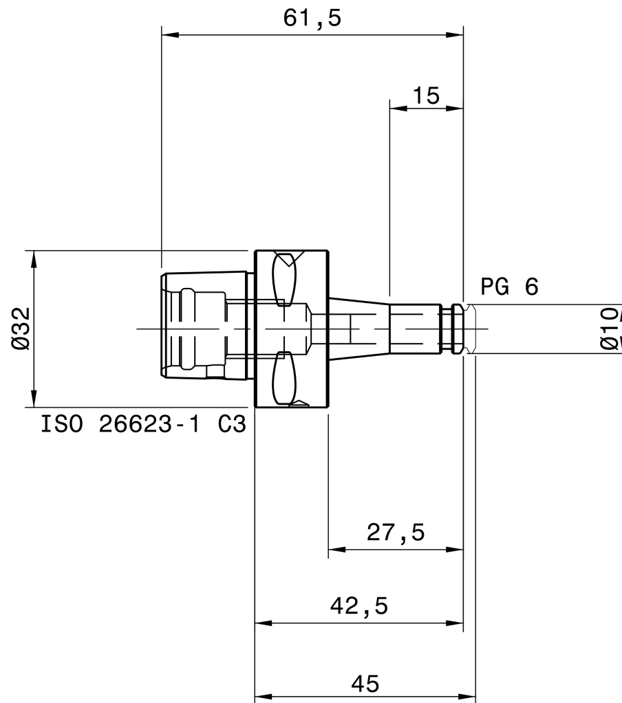
REGO-FIX 2803.70610
