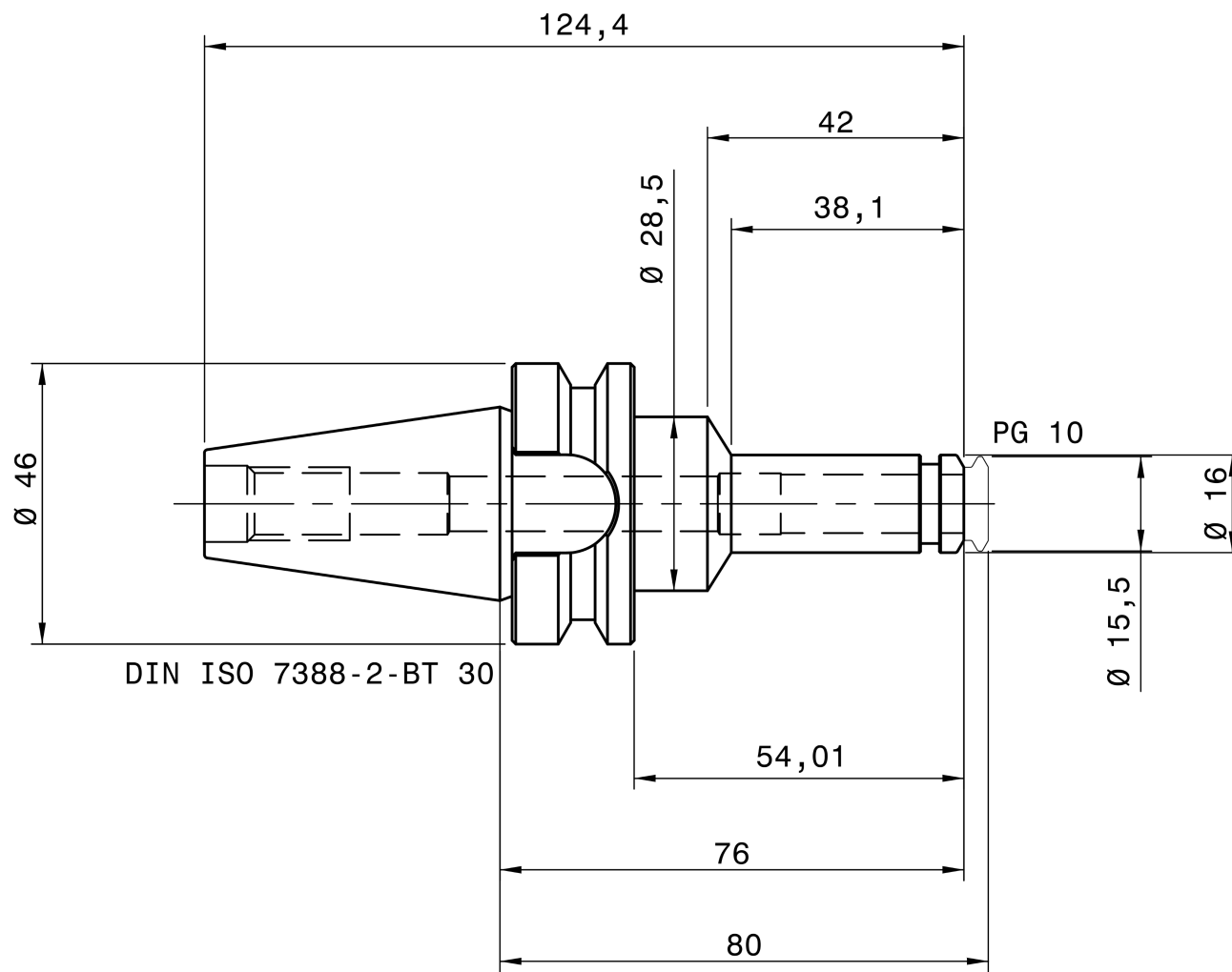
REGO-FIX 4130.71040
