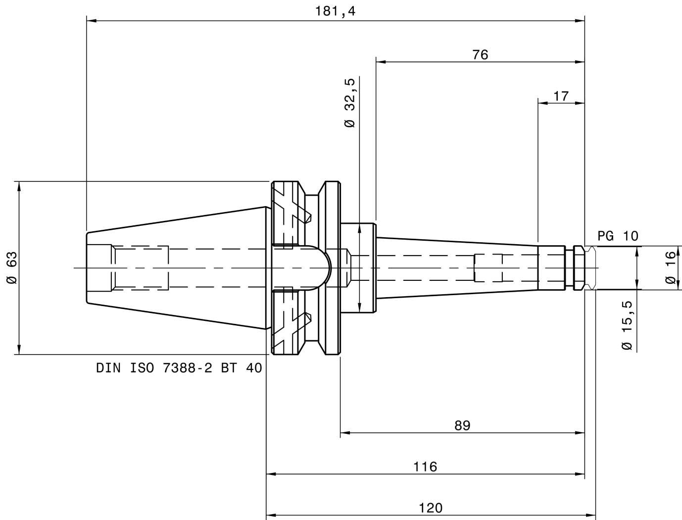
REGO-FIX B 4140.71063
