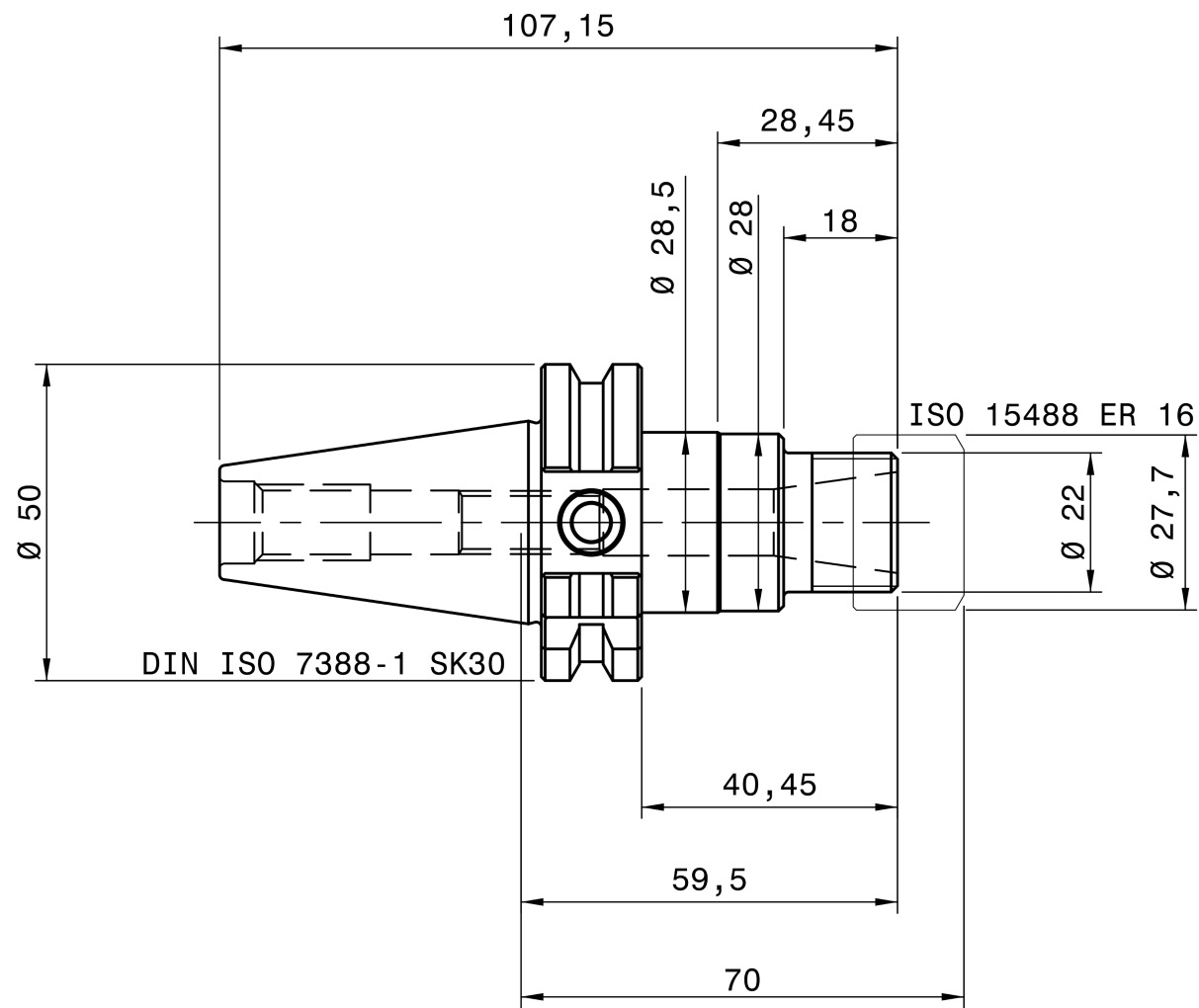
REGO-FIX 4230.11630
