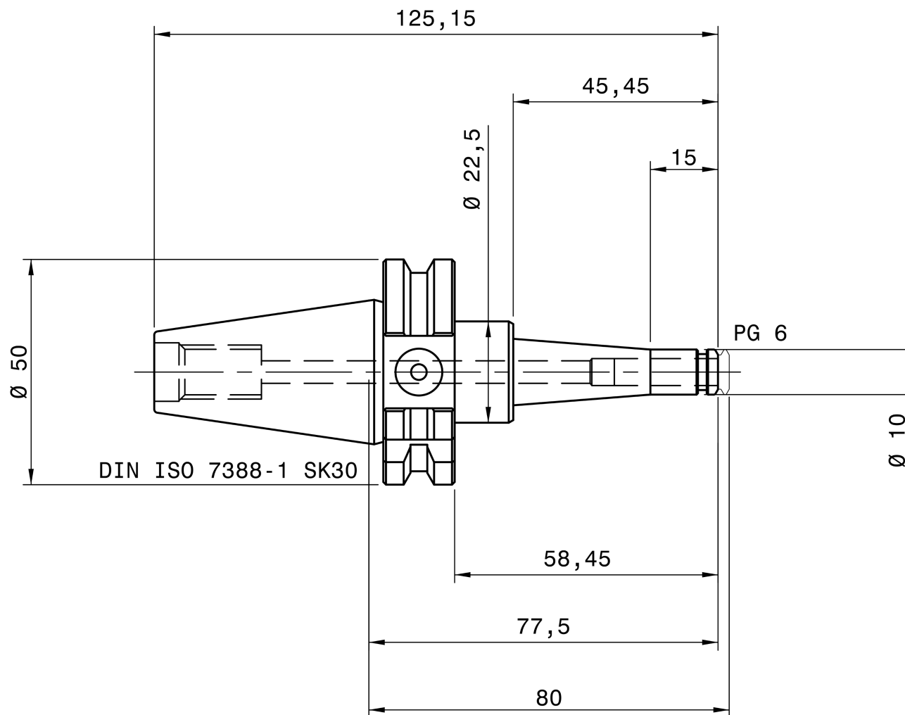
REGO-FIX 4230.70640
