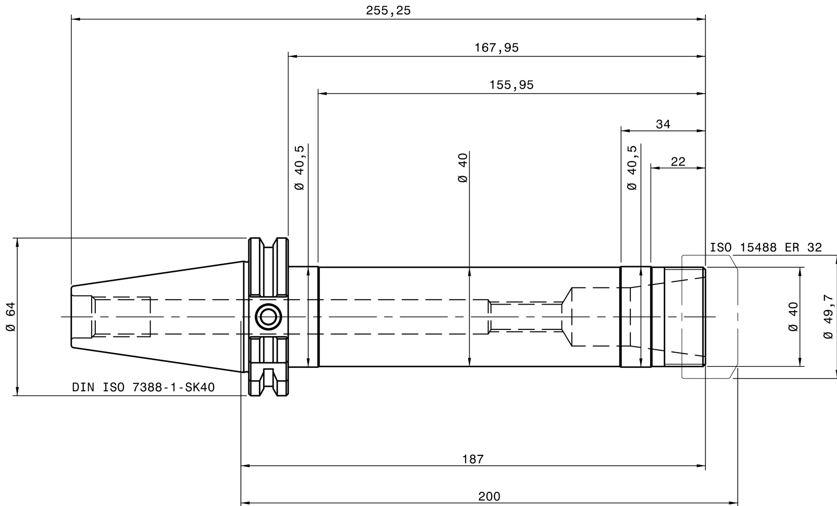
REGO-FIX B 4240.13293
