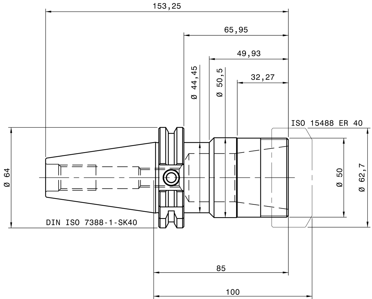
REGO-FIX B 4240.14053
