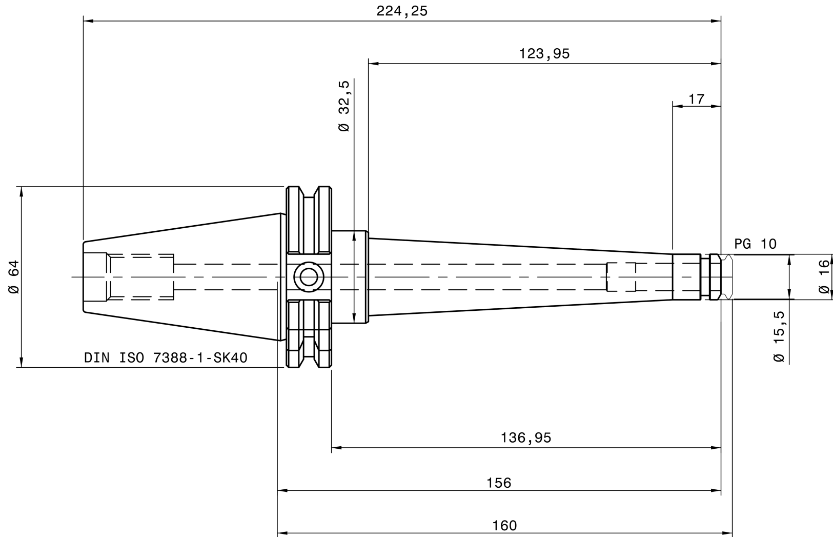
REGO-FIX 4240.71080
