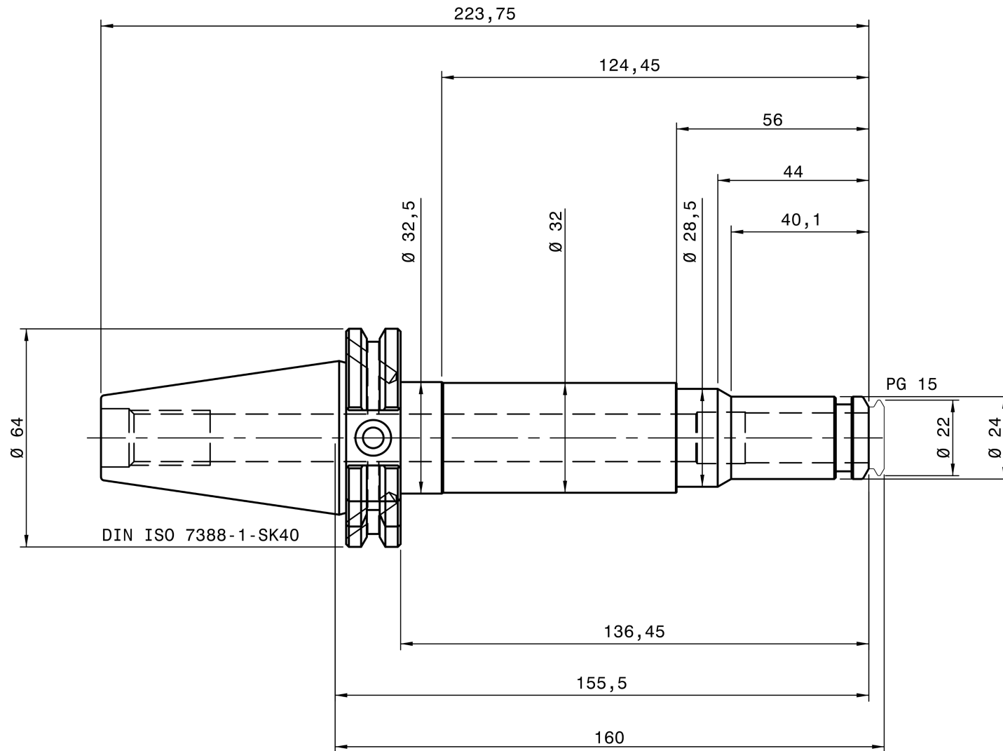
REGO-FIX B 4240.71583
