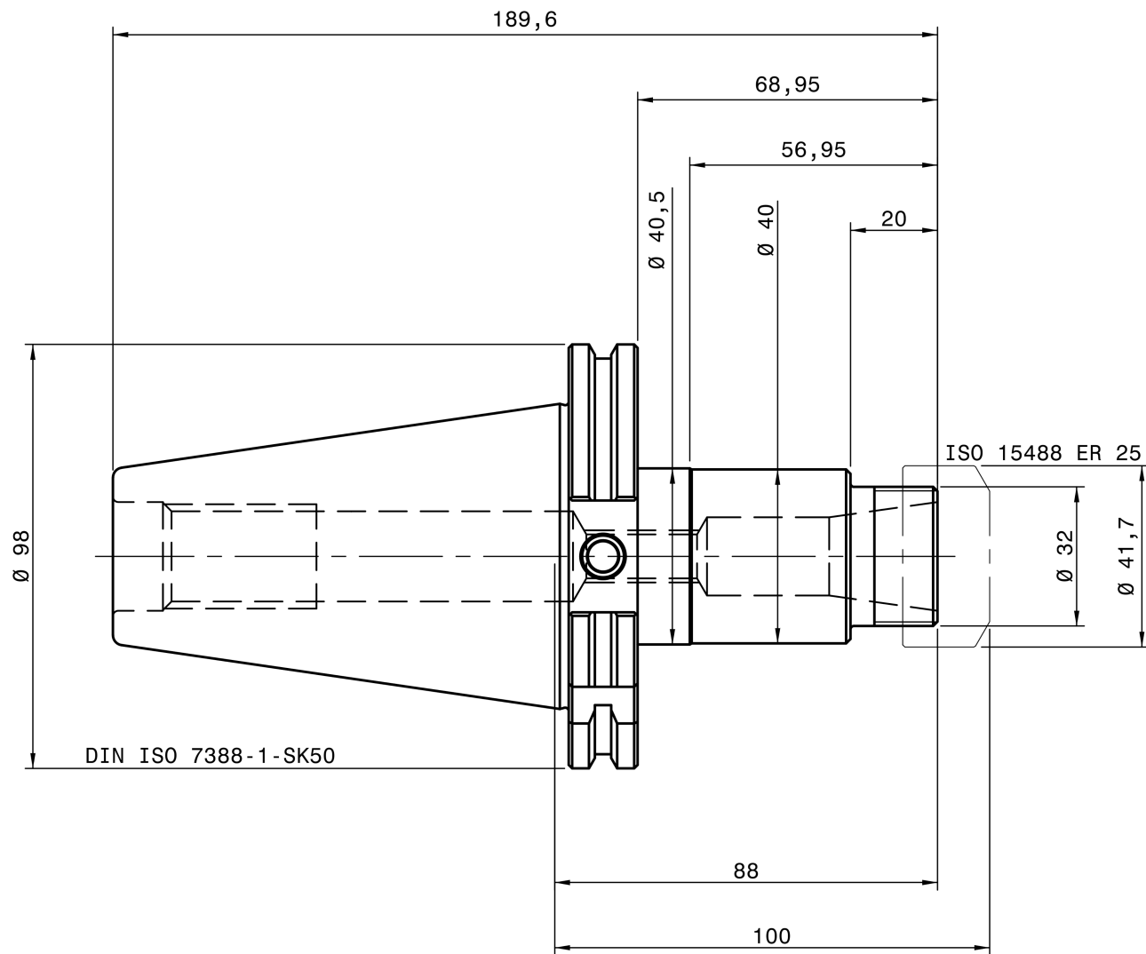
REGO-FIX B 4250.12553
