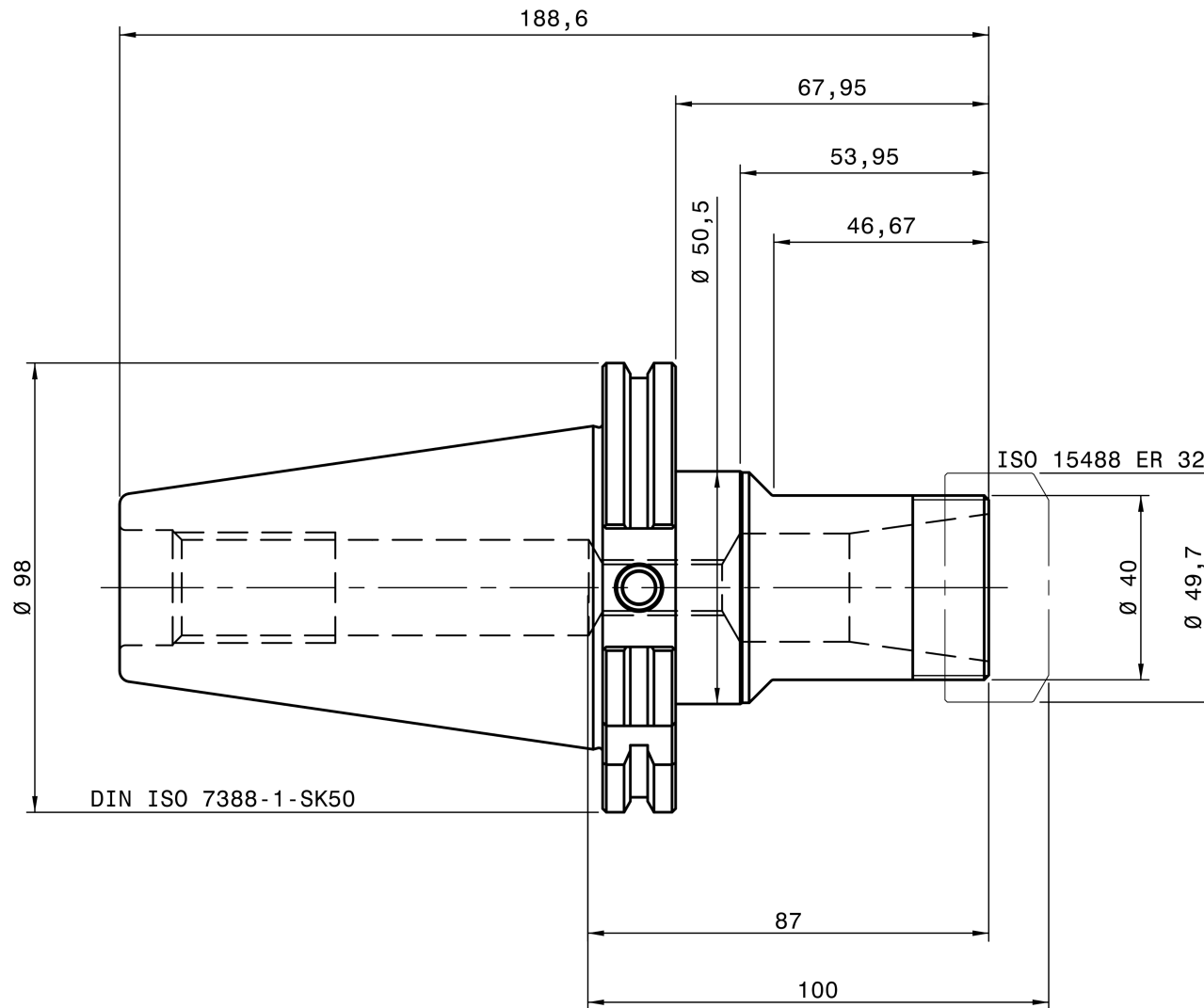
REGO-FIX B 4250.13253
