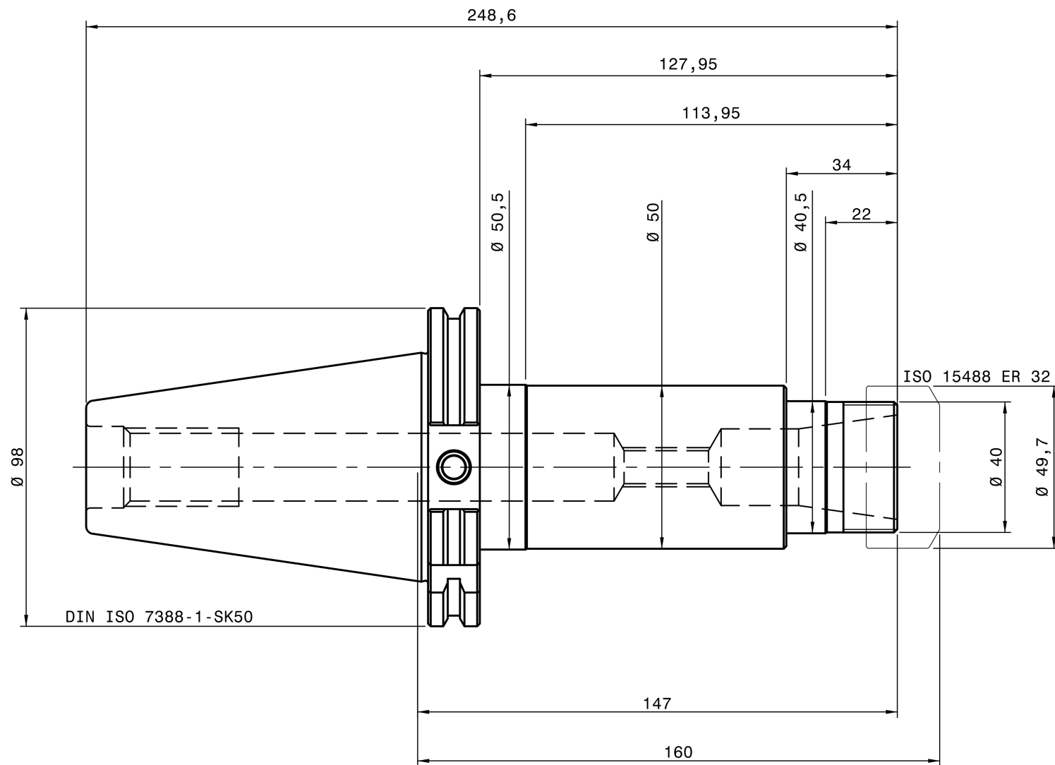
REGO-FIX B 4250.13283
