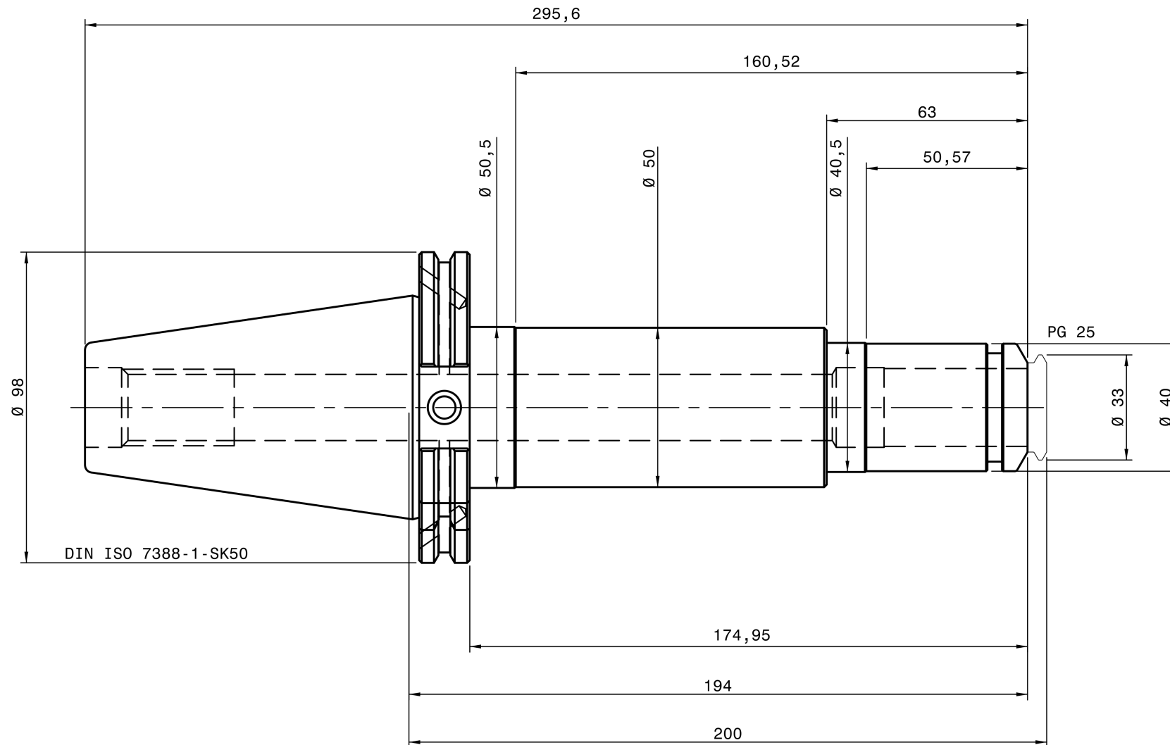
REGO-FIX B 4250.72593
