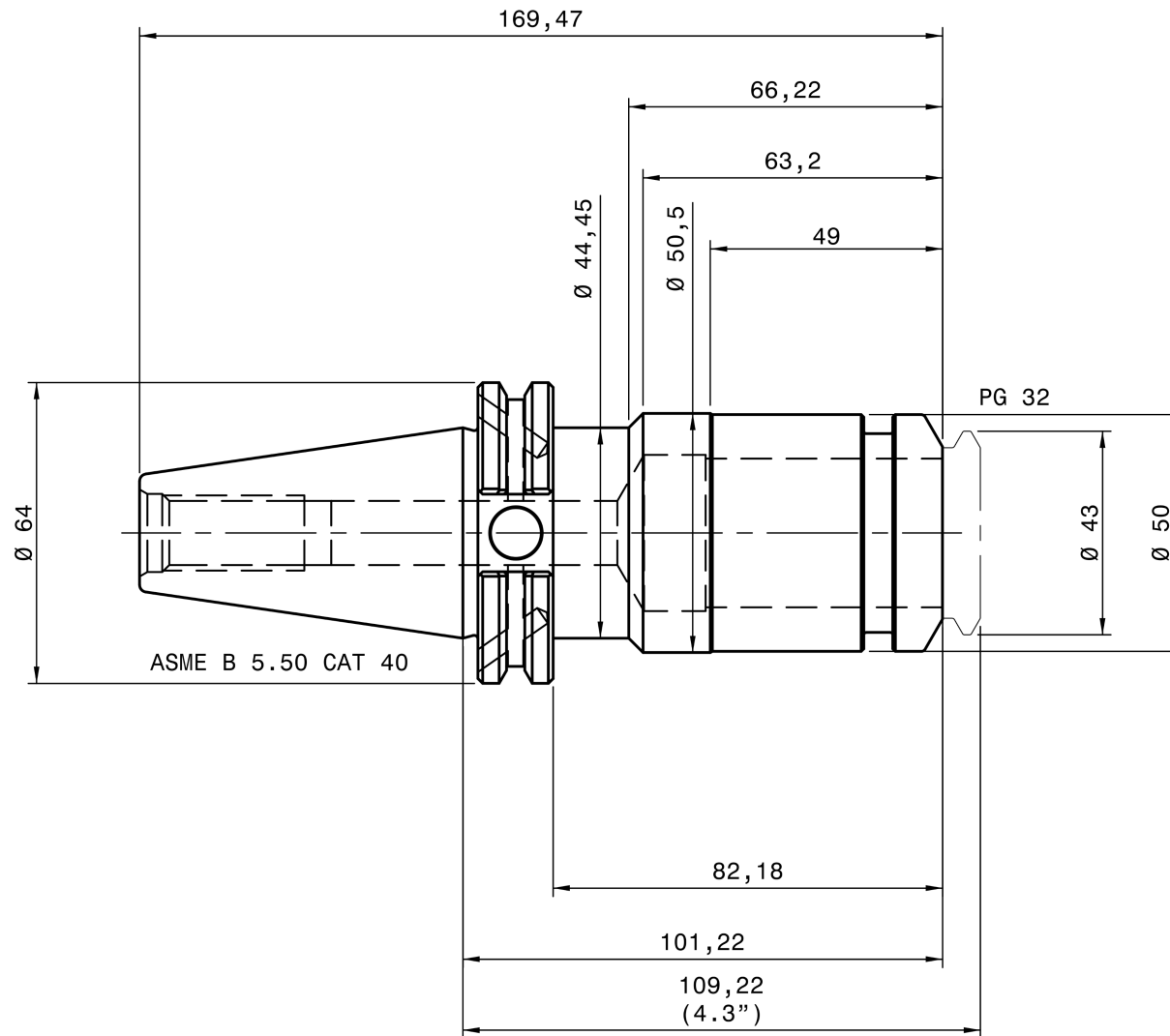
REGO-FIX B 4340.73254
