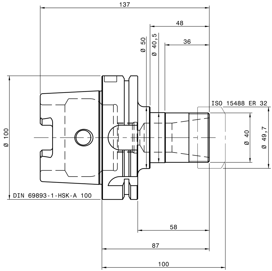
REGO-FIX 4500.13250
