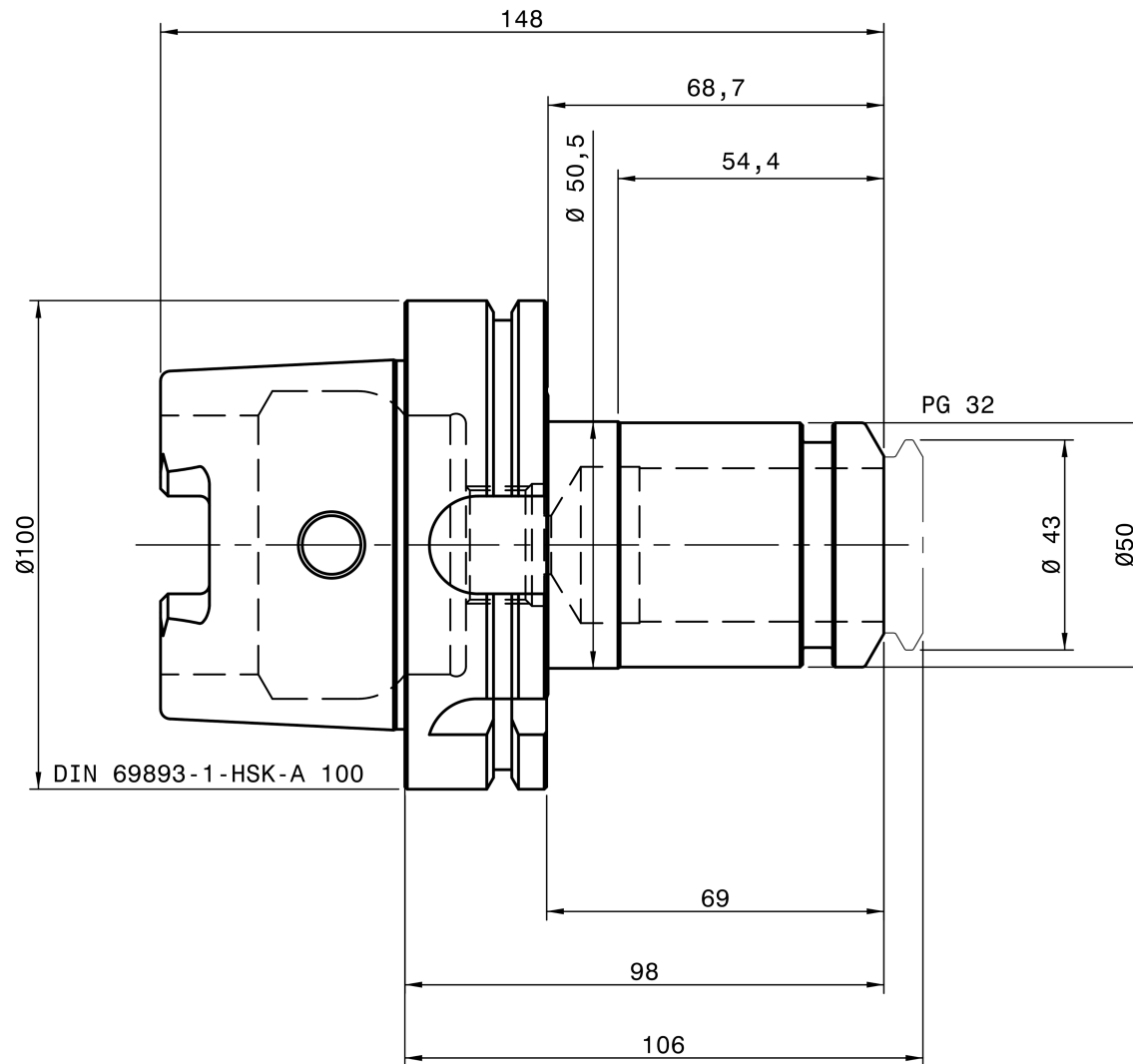
REGO-FIX 4500.73250
