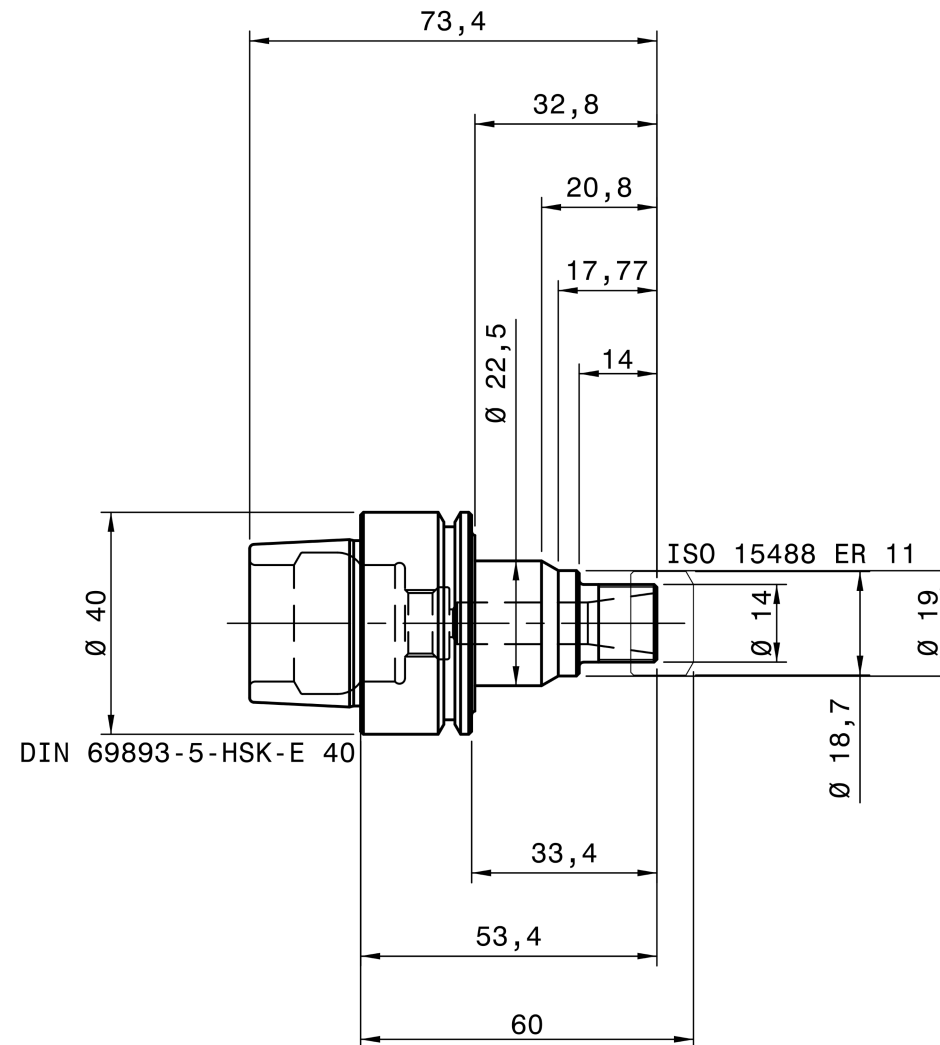
REGO-FIX 4540.11124
