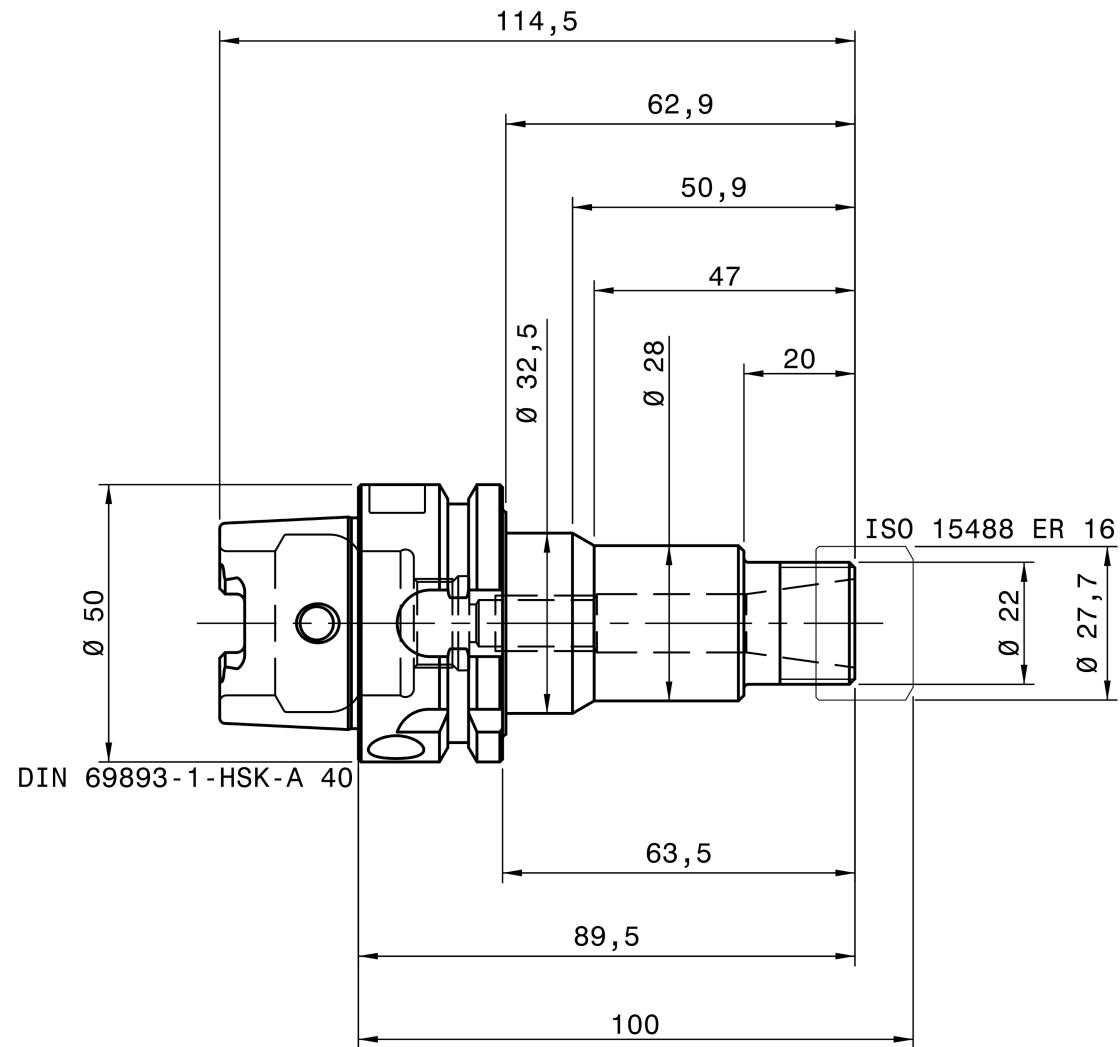
REGO-FIX 4550.11650
