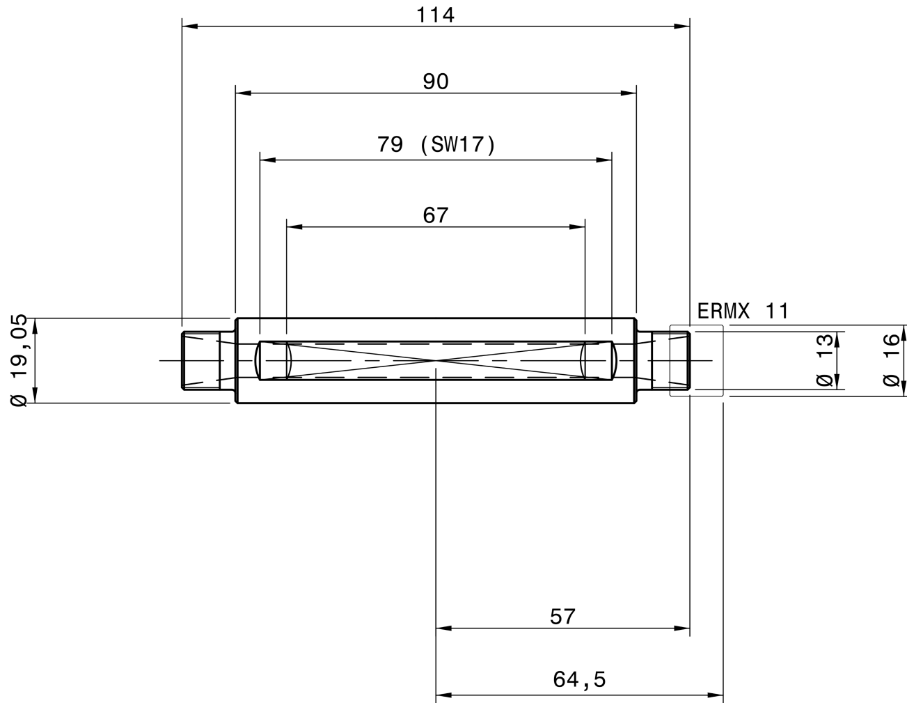
REGO-FIX 4619.21165
