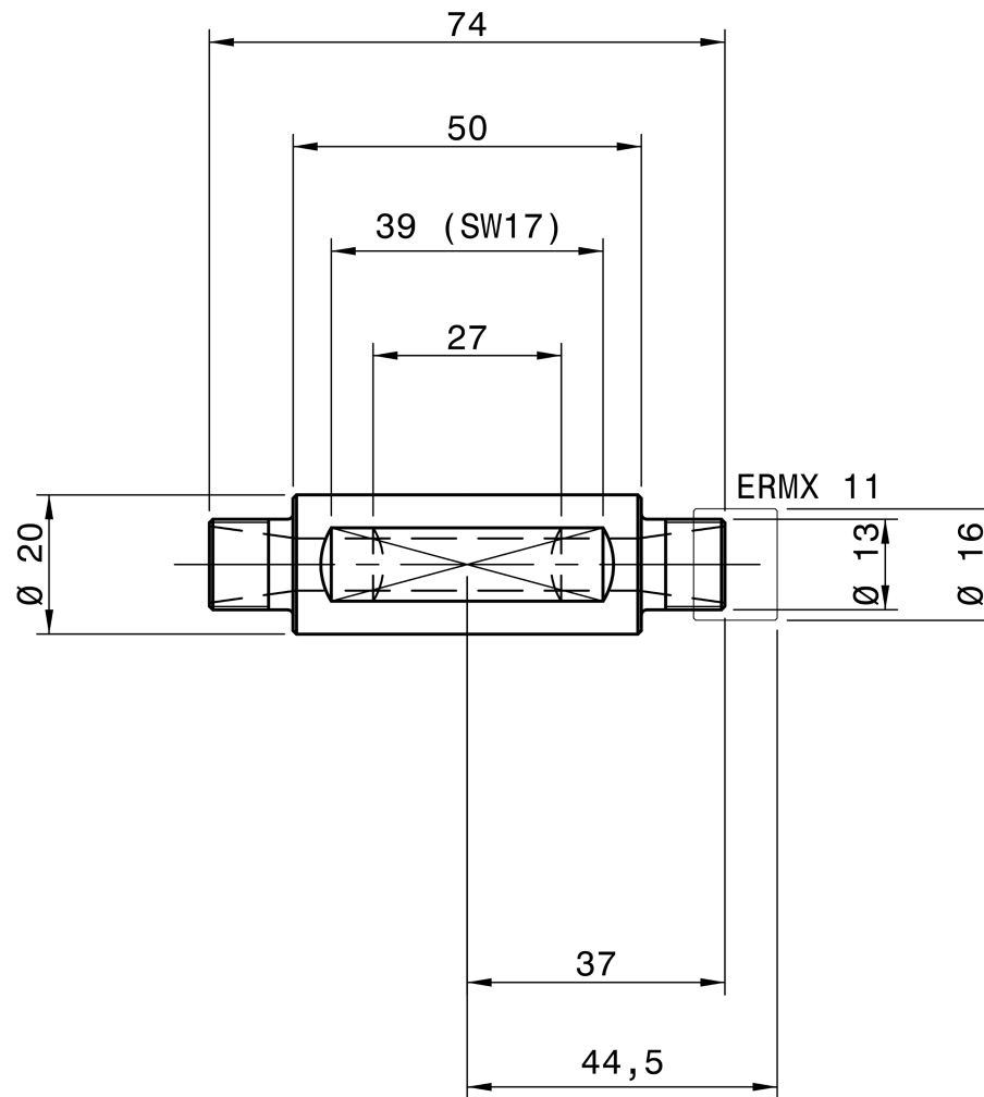
REGO-FIX 4620.21124
