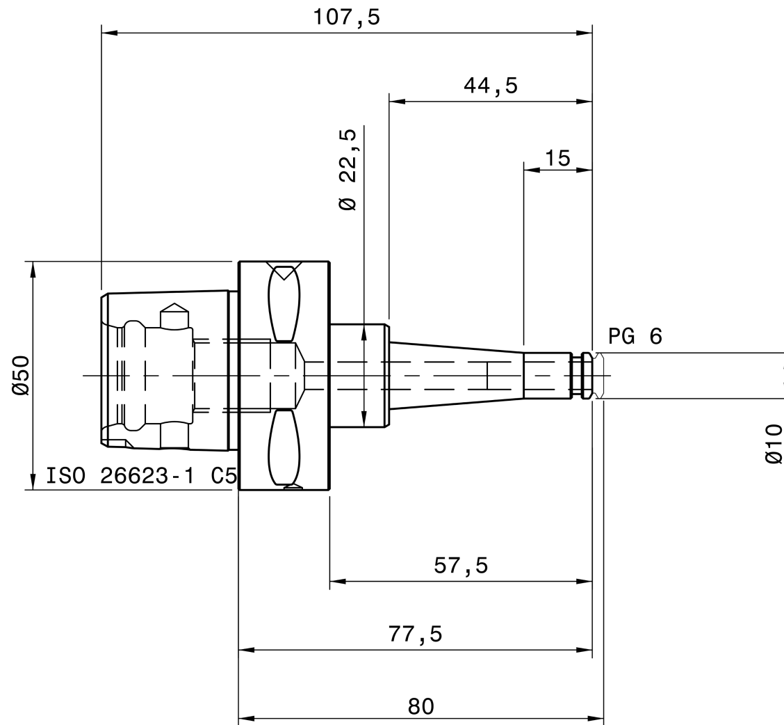
REGO-FIX 4805.70640
