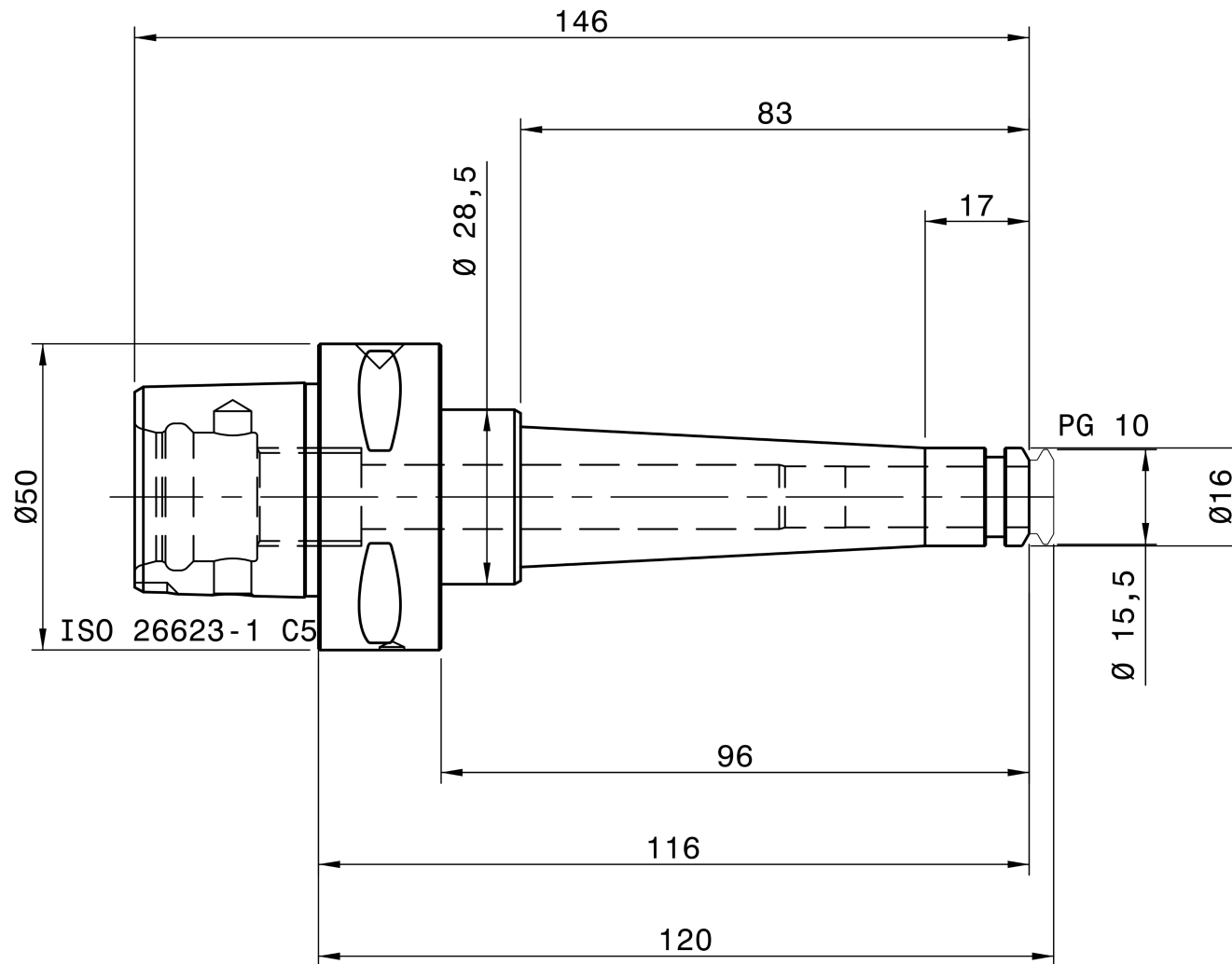
REGO-FIX 4805.71060
