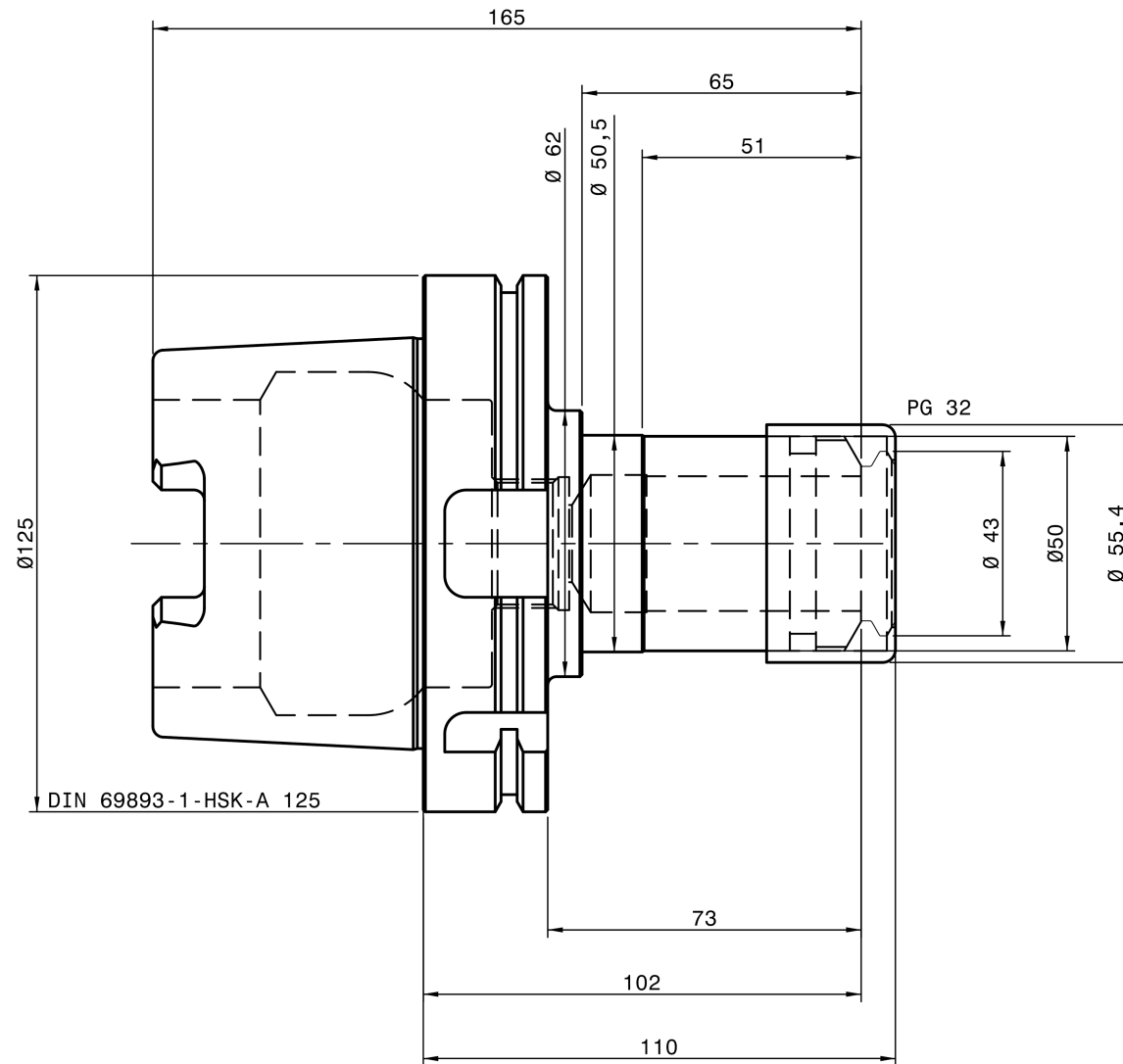
REGO-FIX SG 5502.73250
