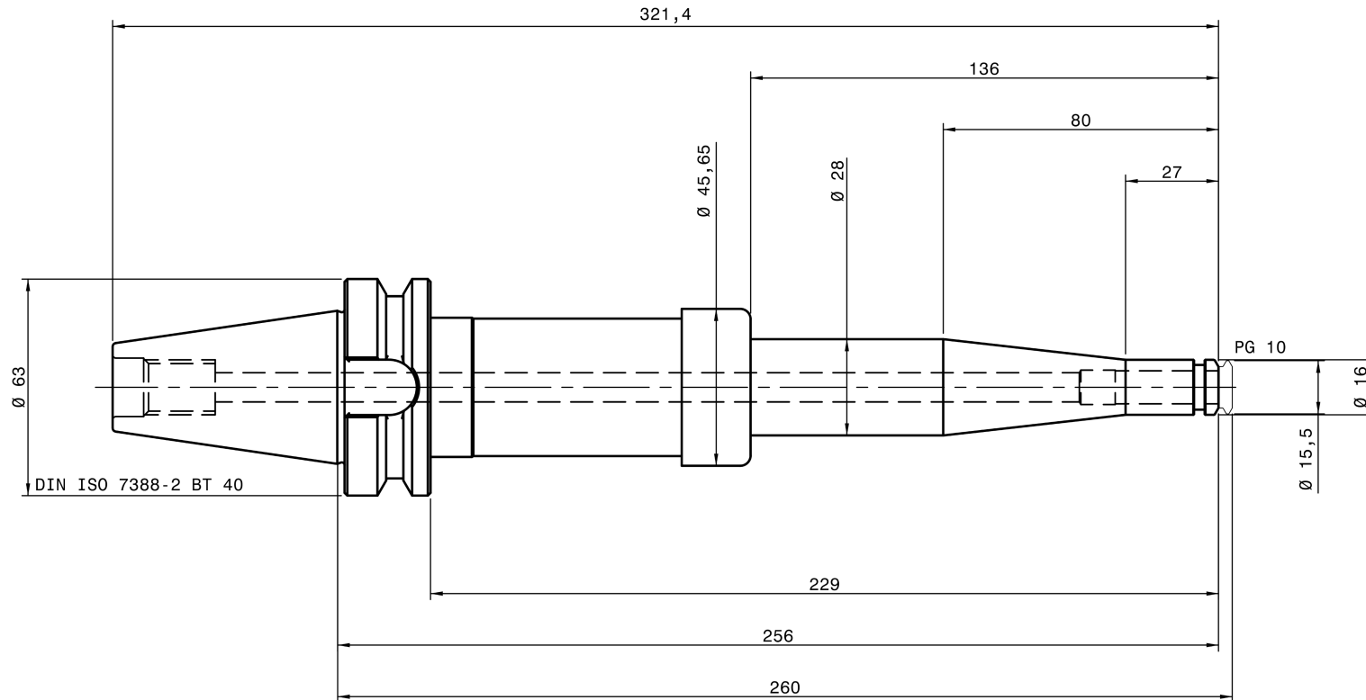
REGO-FIX 8841.71090
