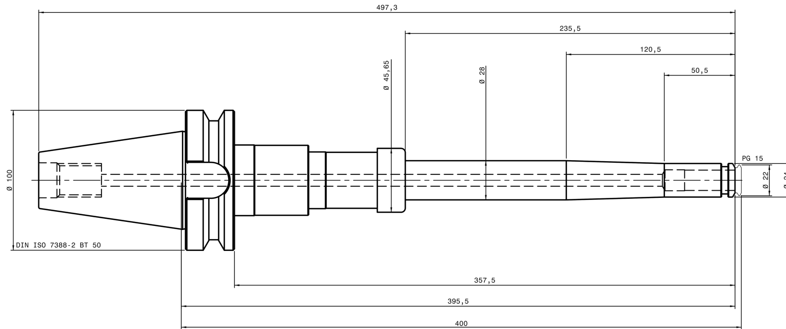
REGO-FIX 8851.73230
