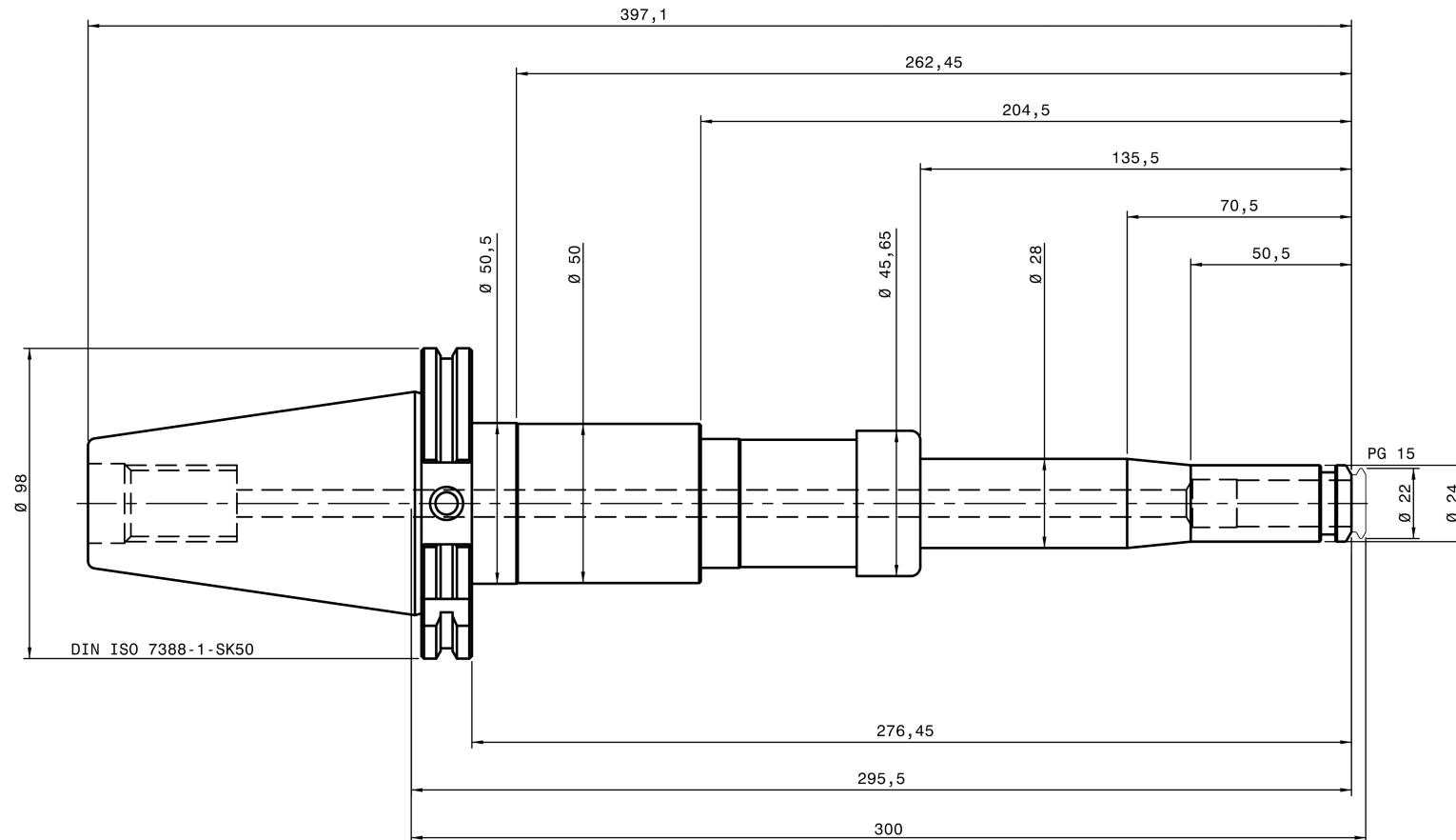
REGO-FIX 8852.73130
