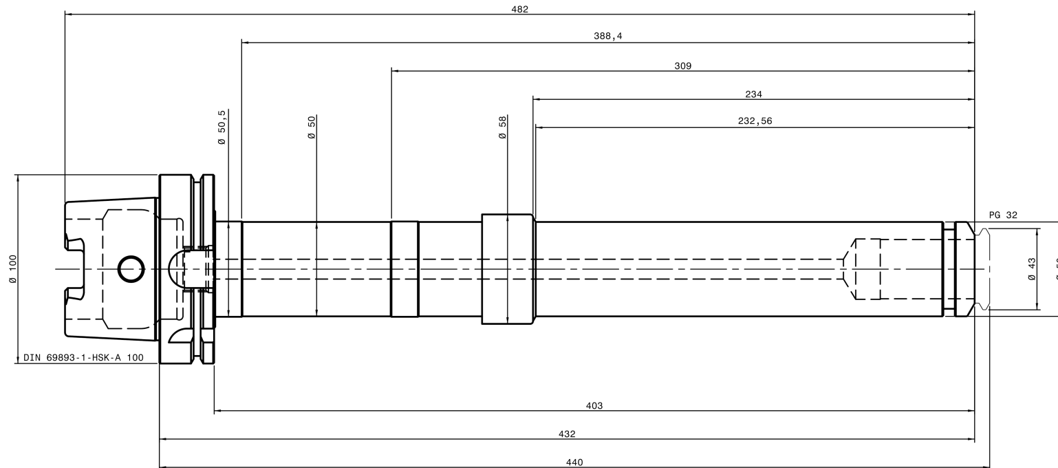
REGO-FIX 8885.78270
