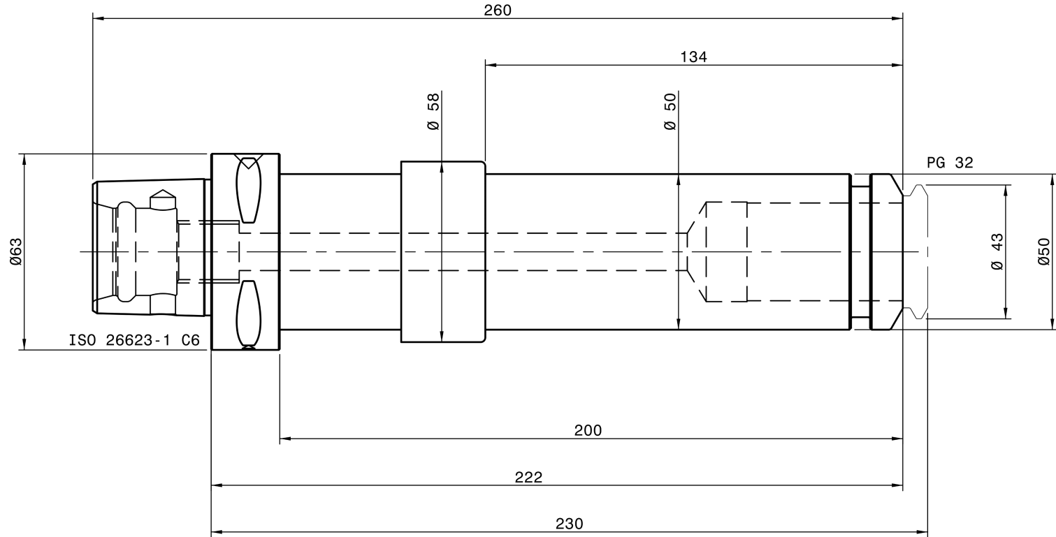
REGO-FIX 8886.78060
